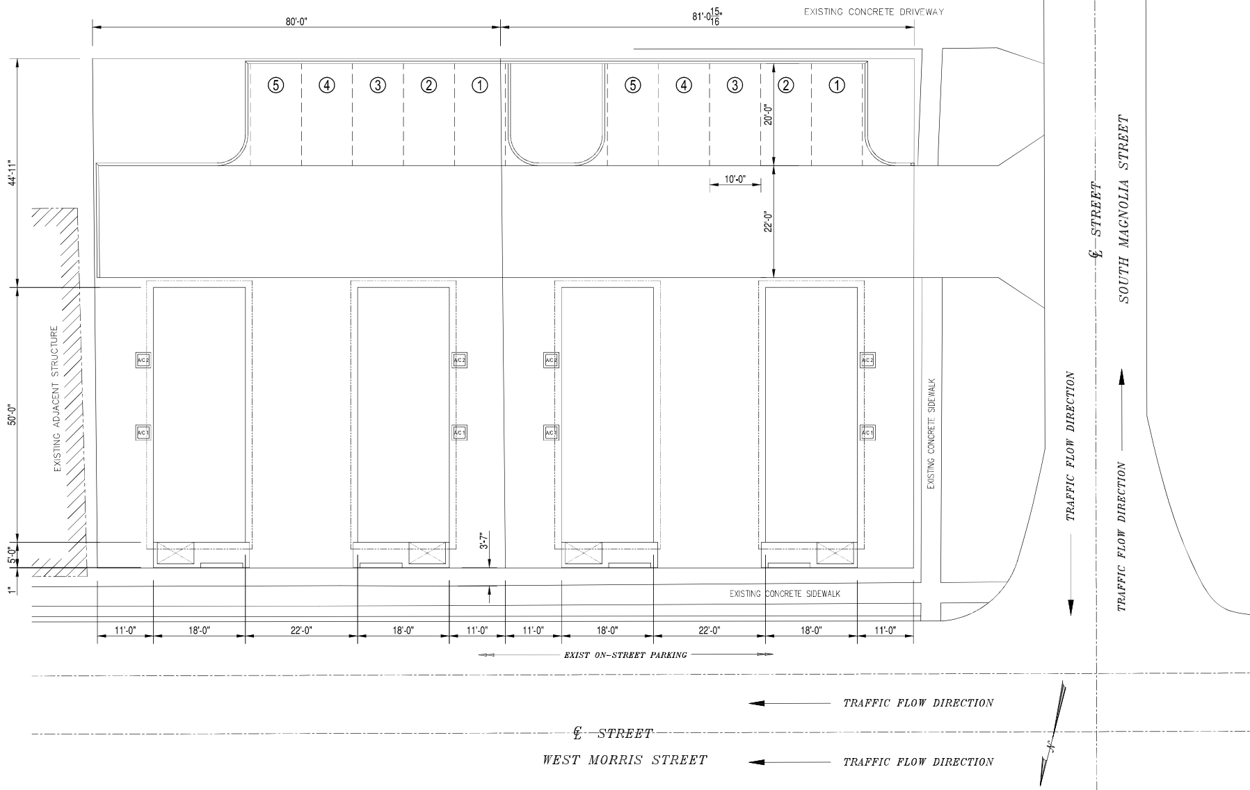
207 - 211 WEST MORRIS REVISED PLOT PLAN - 01/16/2019 SCALE: 1/8" = 1'-0"
