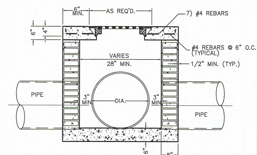
D CATCH BASIN DETAILS
